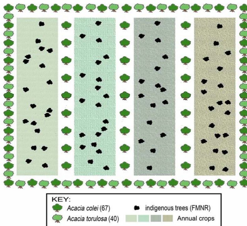
Figure 2. The Farmer Managed Agro-forestry Farming System, one hectare model. Trees on the boundary are spaced 5 m apart. Trees inside the borders are planted 10 m apart in rows with 25 m between rows. The rows of trees are oriented across the prevailing wind direction. Total number of acacia trees =107 per ha. Shaded area: FMNR with 40 to 120 trees per ha and annual/perennial crops in rotation.
